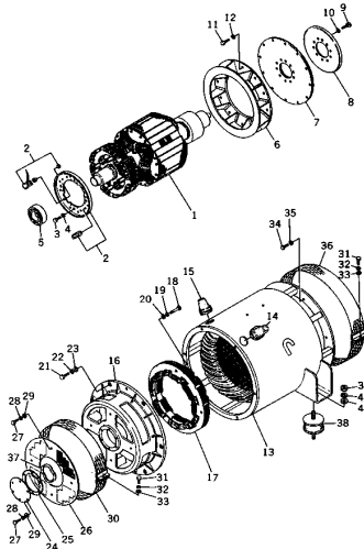
發電機組立圖 (EG125B SERIAL NO. 4001- ) (EXCEPT JAPAN) FIG. 1001 GENERATOR ASS'Y (EG125B SERIAL NO. 4001- ) (EXCEPT JAPAN)
