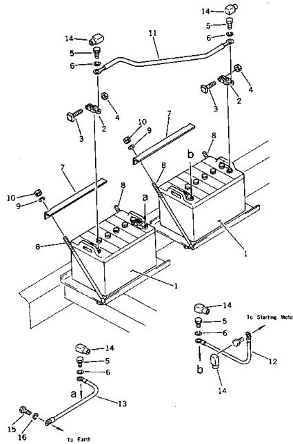
Fig. 141 BATTERY AND CABLE (EG125 Serial No. 1001~)
