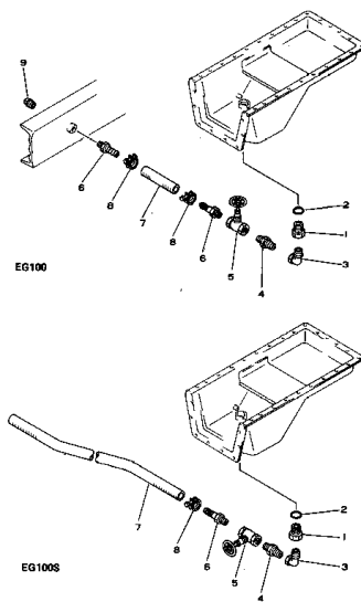
Fig. 161 OIL DRAIN PIPING
