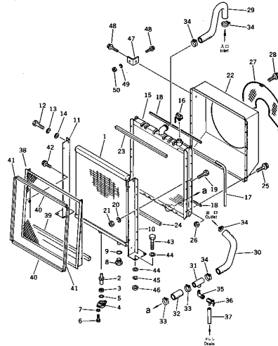
Fig. 121A RADIATOR {EC75Z Serial No. 1197~} {EC75ZS Serial No. 1116~}
