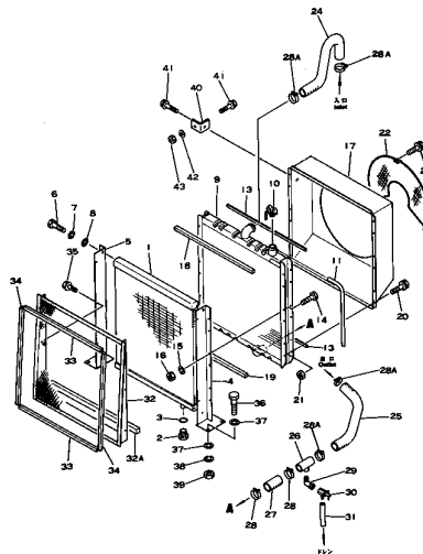
Fig. 121 RADIATOR (EC75Z Serial No. 1001~1196) (EC75ZS Serial No. 1001~1115)
