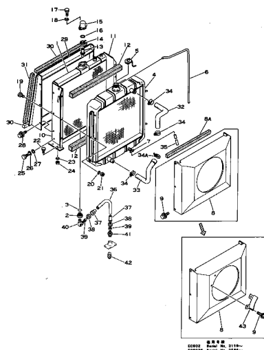
Fig. 121A RADIATOR AND OIL COOLER (EC50Z Serial No. 3001~) (EC50ZS Serial No. 3001~)
