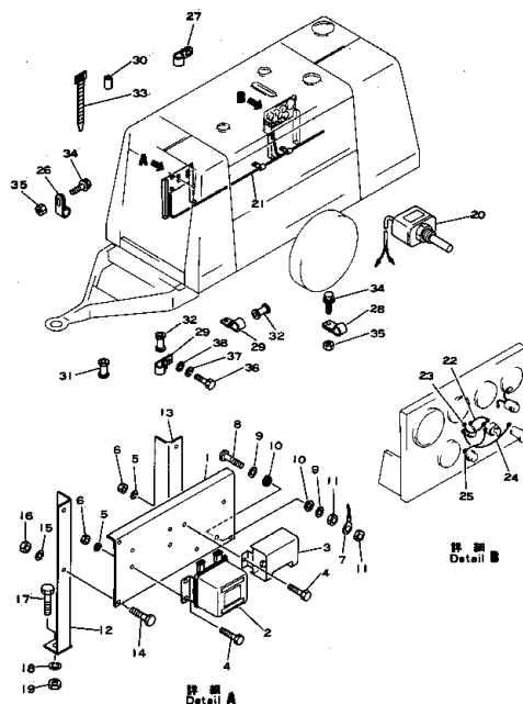
Fig. 151 ELECTRICAL SYSTEM
