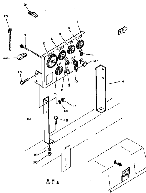
Fig. 145 INSTRUMENT PANEL
