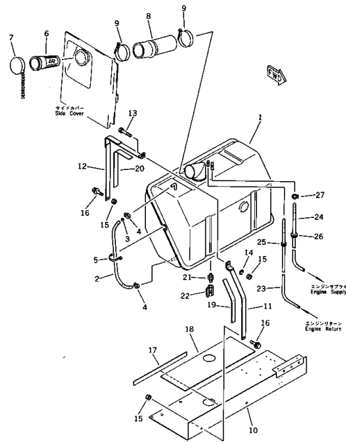
Fig. 131 FUEL TANK (EC35Z Serial No. 1001~) (EC35ZS Serial No. 1001~) (Except Japan)
