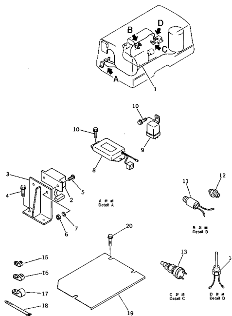
Fig. 151A ELECTRICAL SYSTEM { EC35Z Serial No. 1106~ } 海外向 { EC35ZS Serial No. 1964~ } (Except Japan)
