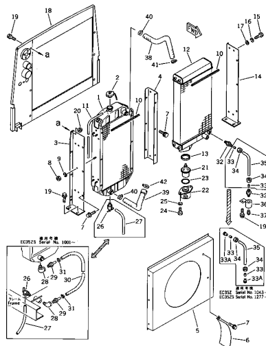
Fig. 121 RADIATOR AND OIL COOLER
