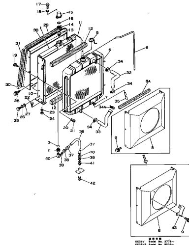
Fig. 121B RADIATOR AND OIL COOLER (EC35V Serial No. 3443~) (EC35VS Serial No. 3763~)
