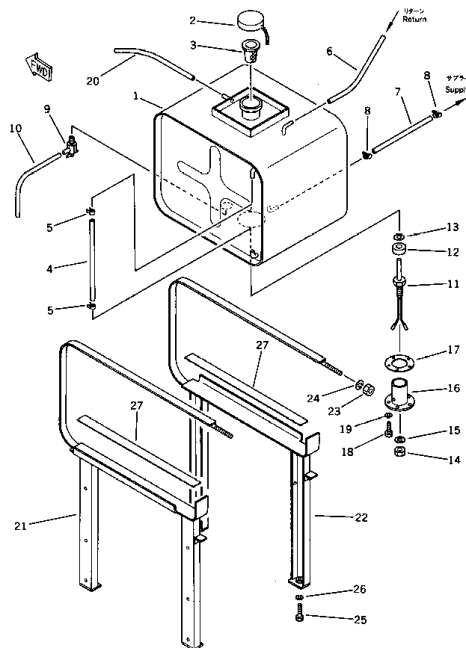
Fig. 131 FUEL TANK
