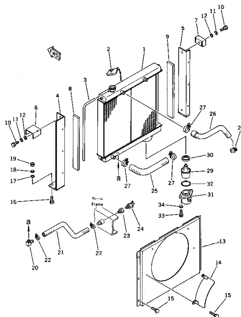
Fig. 121 RADIATOR AND OIL COOLER
