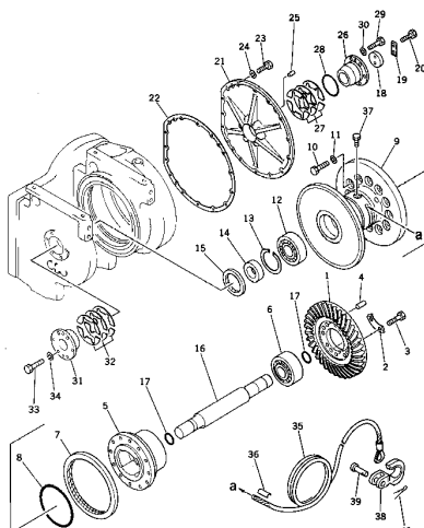
Fig. 204 BEVEL GEAR AND DRUM
