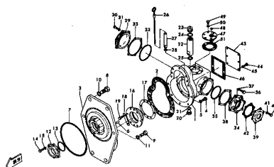
Fig. 101 DRIVE GEAR CASE
