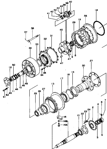
Fig. 121A DRUM, L.H. (Serial No. 2001~)
