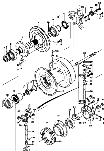
Fig. T03 BEVEL GEAR, CLUTCH AND DRUM
