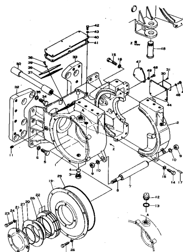
Fig. 101 CASE (1/4)
