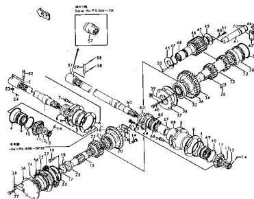
Fig. 103 POWER TRANSMISSION (2/2) (適用号機 Serial No. (16001)~1756)
