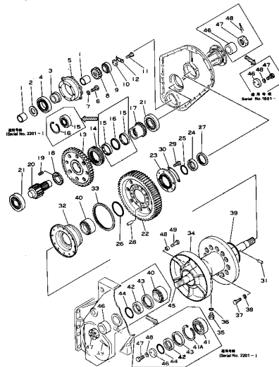
Fig. 104 GEAR AND DRUM
