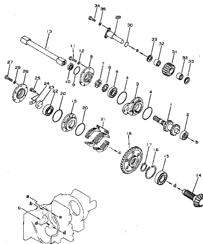
Fig. 102 P.T.O. SHAFT AND GEAR
