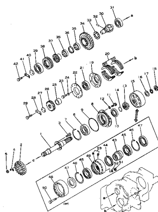
Fig. 103 GEAR AND BRAKE DRUM
