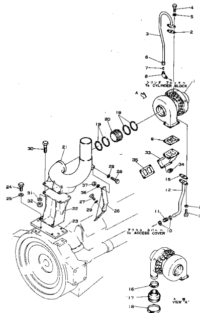
Fig.104 TURBOCHARGER CONNECTION
