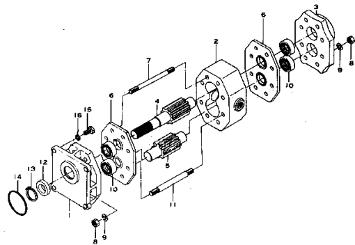
FIG. 114 HYDRAULIC PUMP (適用号機 Serial No. D (6001~9999))
