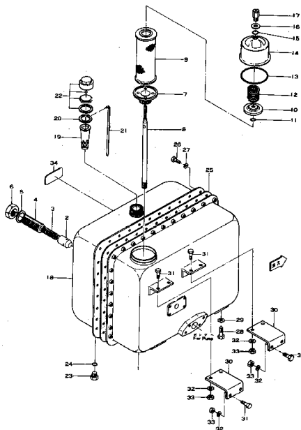
FIG. 115 HYDRAULIC TANK (適用号数 Serial No. D (6001~9999))
