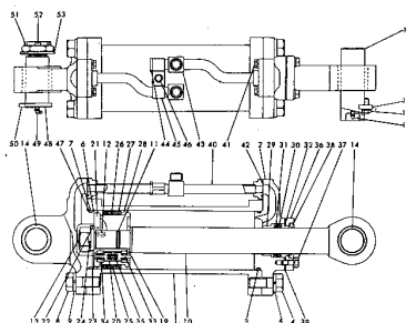
Fig. 112 HYDRAULIC CYLINDER (Serial No. D50S (5861)-(15400))
