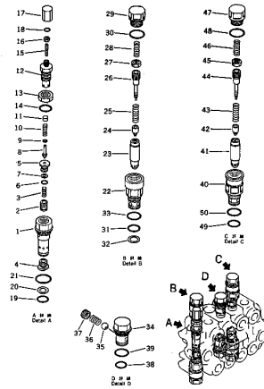
Fig. 233 HYDRAULIC CONTROL VALVE(3/3) (D31A Serial No. 1001~)
