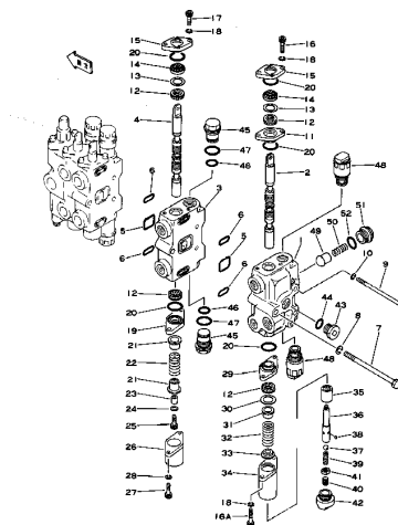
Fig. 135 HYDRAULIC CONTROL VALVE(1/3) (D31A Serial No. 2001~)
