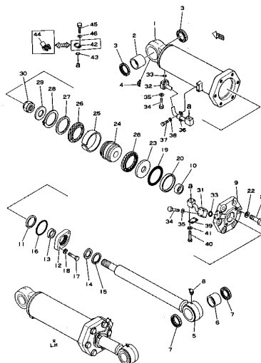
Fig.111B RIPPER CYLINDER (Serial No. 3301-)
