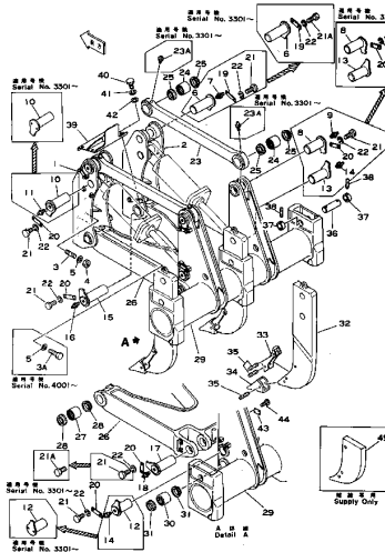
Fig.101A RIPPER SHANK, BEAM AND LINK (Serial No. 1632 ~)
