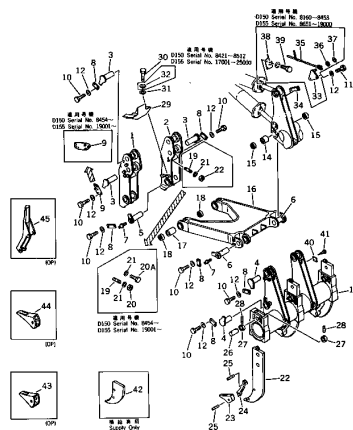
Fig. 201B RIPPER SHANK, BEAM AND LINK (D150 Serial No. 8421~) (D155 Serial No. 17001~)
