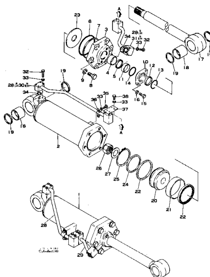
Fig. 111A LIFT CYLINDER (D150 Serial No. 8329~8420) (D155 Serial No. 10263~17000)
