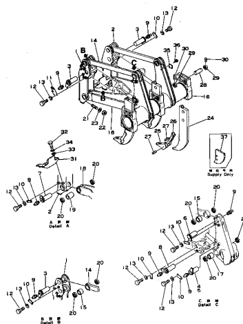
Fig. 101A RIPPER SHANK, BEAM AND LINK (D150 Serial No. 8329~8420) (D155 Serial No. 10263~17000)
