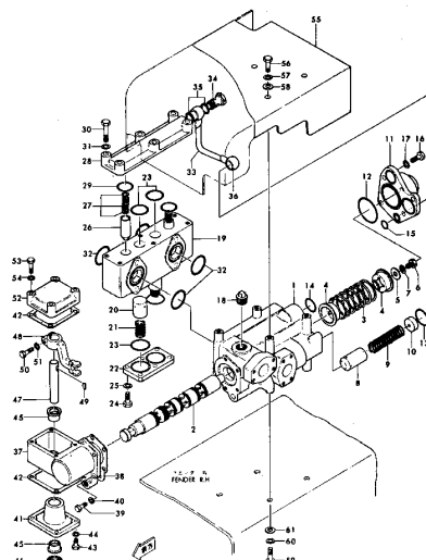
FIG. 1.03 CONTROL VALVE (Hydraulic Type, D120A-8,15,18 AND D125A-18)
