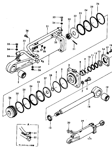
FIG. 102 HYDRAULIC CYLINDER
