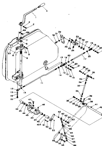
Fig.563 CONTROL LEVER
