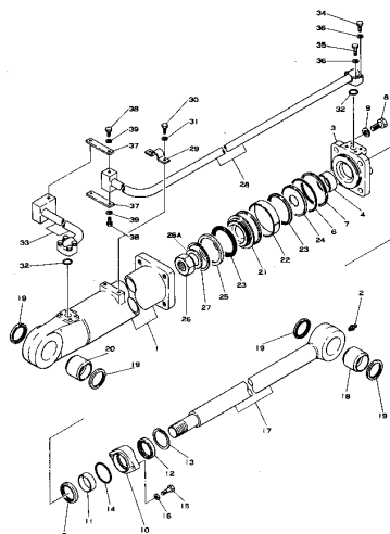
Fig.518 030010 HYDRAULIC CYLINDER
