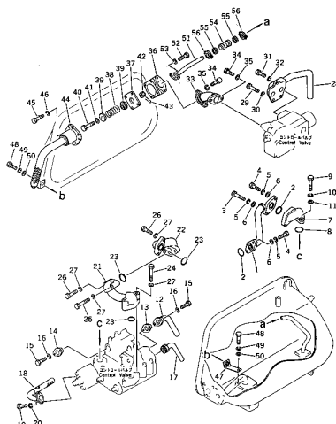
Fig. 132 HYDRAULIC TANK(2/3)
