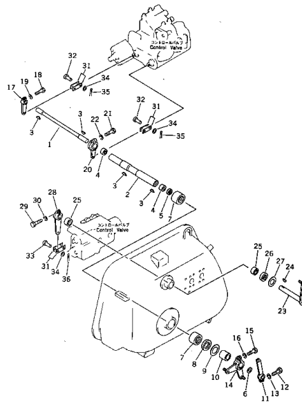
Fig. 133 HYDRAULIC TANK(3/3)
