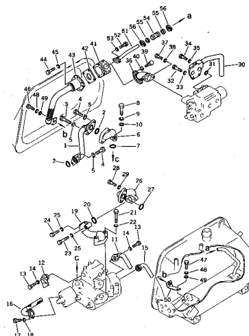
Fig. 136 HYDRAULIC TANK(2/3) (D60-65S Serial No. 40001~)
