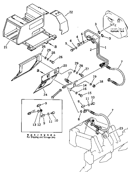
Fig. 121 HYDRAULIC PIPING
