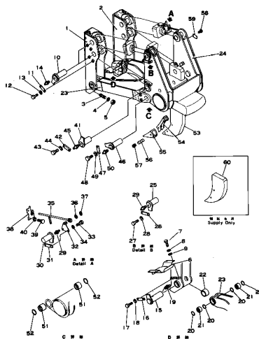
Fig. 201 RIPPER SHANK, BEAM AND LINK (D150 Serial No. 6843~8328) (D155 Serial No. 6843~10262)
