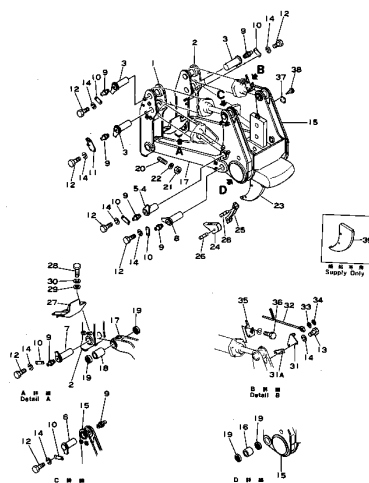
Fig. 201A RIPPER SHANK, BEAM AND LINK (D150 Serial No. 8329~8420) (D155 Serial No. 10263~17000)
