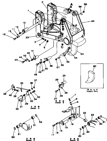
Fig. 201 RIPPER SHANK, BEAM AND LINK (D150 Serial No. 6843~8328) (D155 Serial No. 6843~10262)
