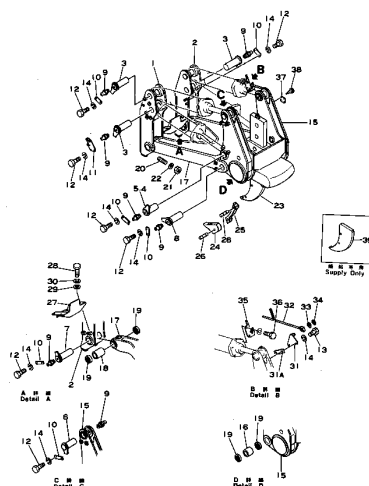
Fig. 201A RIPPER SHANK, BEAM AND LINK (D150 Serial No. 8329~8420) (D155 Serial No. 10263~17000)
