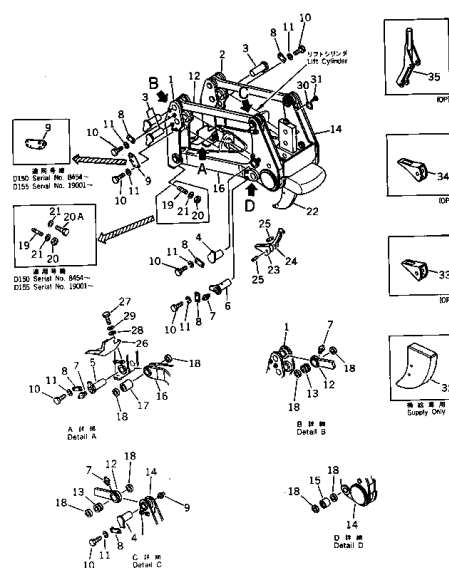
Fig. 101B RIPPER SHANK, BEAM AND LINK (適用機種: D150 Serial No. 8421~ D155 Serial No. 17001~)
