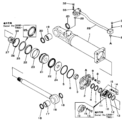
Fig. 111 LIFT CYLINDER (適用機種) (D150 Serial No. 5508~8328) (D155 Serial No. 5508~10262)
