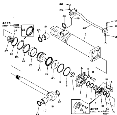
リフトシリンダ (適用機種) Fig. 111 LIFT CYLINDER (D150 Serial No. 5508~8328 (D155 Serial No. 5508~10262))
