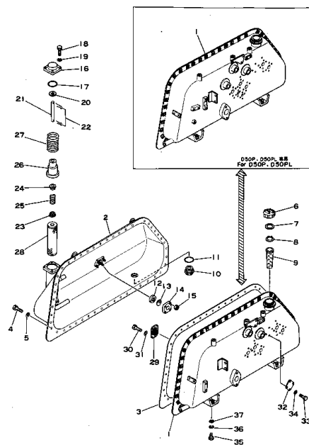
Fig. 121 HYDRAULIC TANK (1/2)
