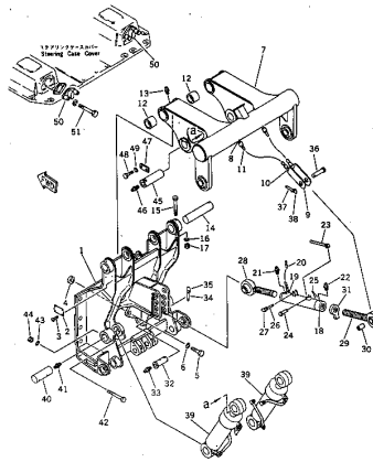
Fig. 201 3-POINT HITCH (1/2)
