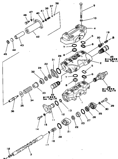
Fig. 1115 3PT. HITCH CONTROL VALVE (1/2)
