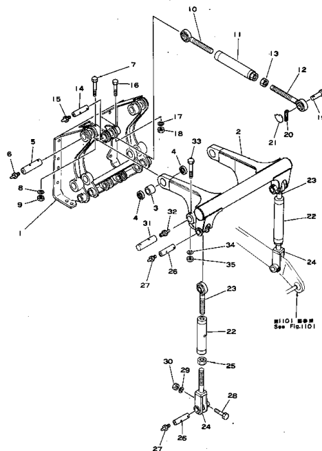
Fig. 1102 3PT. HITCH (2/2)
