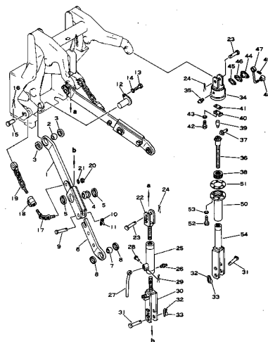
Fig. 102A 3-POINT HITCH (2/2) (DNH031-2 Serial No. 2001~)
