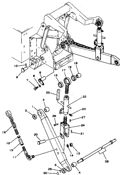
3 点 ヒッチ (2/2) (DNH031-1 Serial No. 2001 ~) Fig. 102 3-POINT HITCH (2/2)
