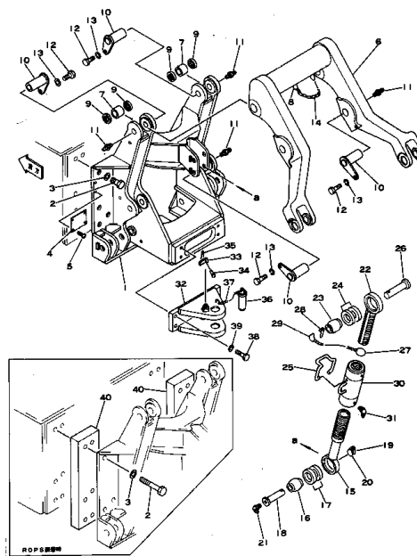
Fig. 101 3-POINT HITCH (1/2) (DNH031-1 通用機種 Serial No. 2001~)
