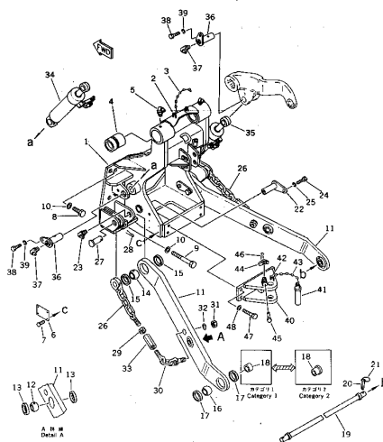
Fig. 3101 3-POINT HITCH (1/2)
