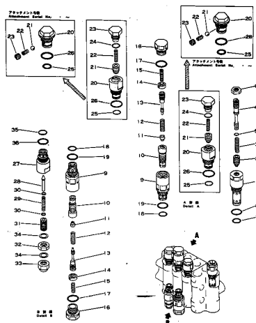
Fig. 3123 HYDRAULIC CONTROL VALVE (3/3) (D20,21A)
