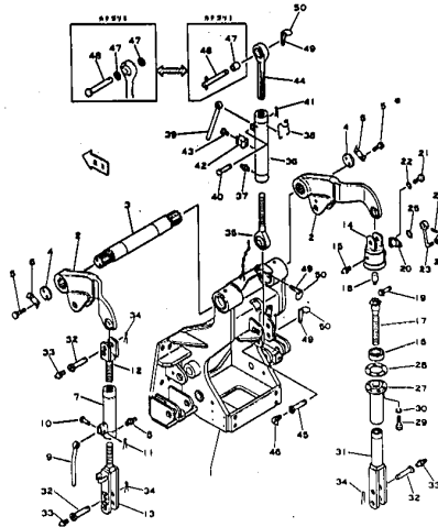
Fig. 3102 3-POINT HITCH (2/2)
