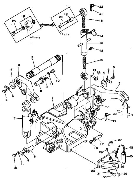
Fig. 202 3-POINT HITCH (2/2)
