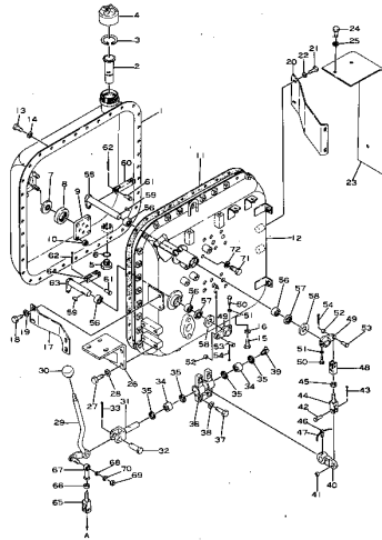
FIG. 131 HYDRAULIC TANK AND 3-POINT HITCH LEVER
