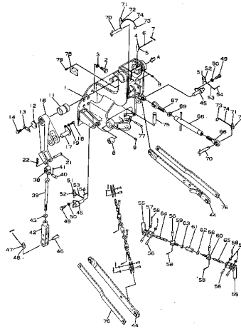
FIG. 101 3-POINT HITCH (1/2)
