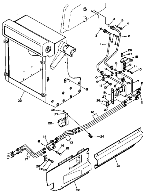
Fig. 121 HYDRAULIC PIPING (1/2)
