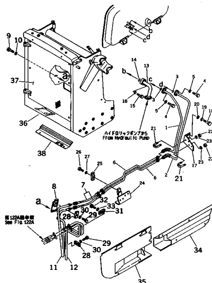
FIG. 121A HYDRAULIC OIL PIPING (1/2) (#(81229)-)
