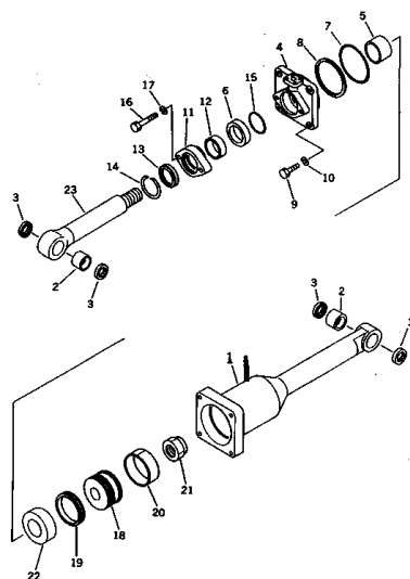
FIG. 111 TILT CYLINDER
