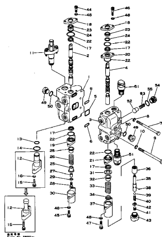
Fig. 125 BLADE CONTROL VALVE (1/2)
