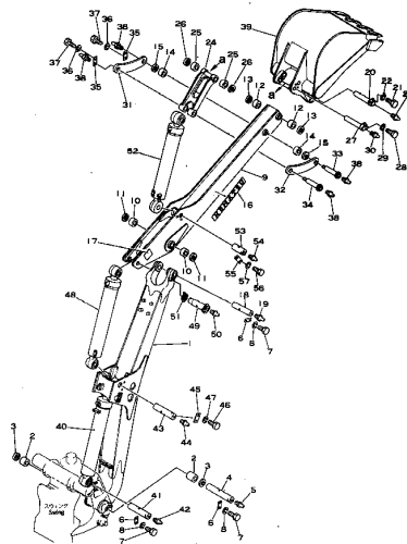
Fig. 101A BOOM (DHS030-C,D,E,F,G,J,K,L,M,N,P,R,S,T,U,V,W,X,Y,Z,B1,C1,D1,E1,G1) (適用機種 Serial No. 6414~)
