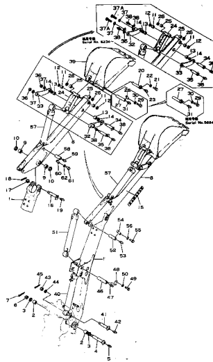
Fig. 101 BOOM (DHS030-C,D,E,F,G,J,K,L,M,N,P,R,S,T,U,V,W) (適用機種 Serial No. 5004-6413)
