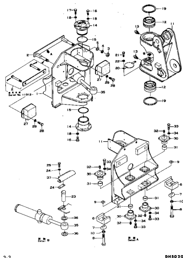
Fig. 201 SWING (Serial No. ABCD 10002~14999)
