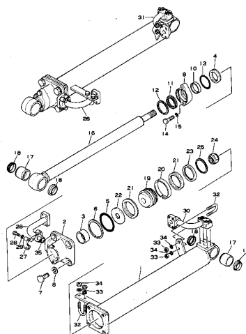
Fig. 111 HYDRAULIC CYLINDER
