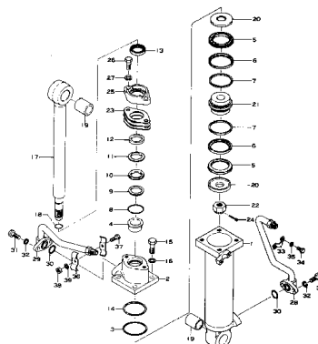
FIG. 111 HYDRAULIC CYLINDER (Serial No. A(20713~30587))
