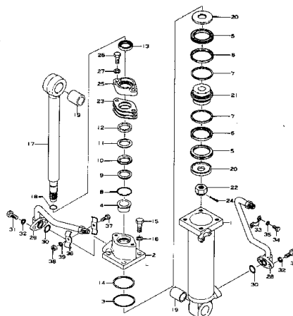
FIG. 113 HYDRAULIC CYLINDER (適用号数 A Serial No. B 1001~)
