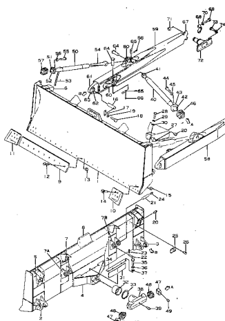
Fig. 101A TILT DOZER (Serial No. 2067~ (29848))
