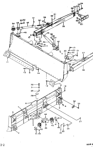
Fig. 101 TILT DOZER (Serial No. 2001~2066)
