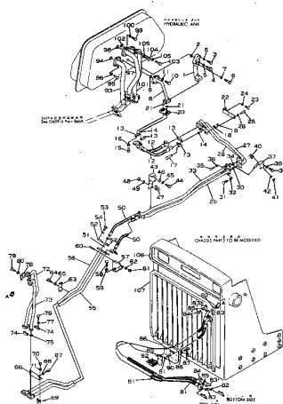
Fig. 121 HYDRAULIC PIPING
